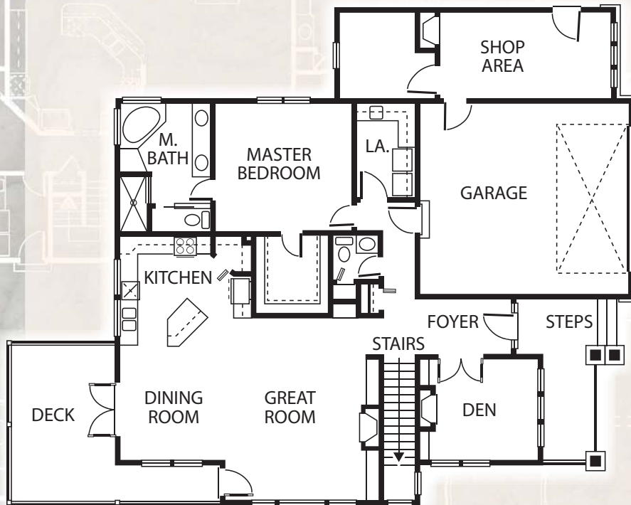
PLAN 1669 RANCHER 52'6 Width x 57' Depth
